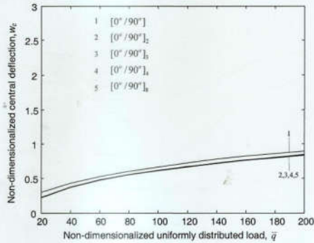
Fig. 3 Number of layers effect on a simply supported (SS5) antisymmetric cross-ply [(0^\circ/90^\circ)_n] square plate under uniformly distributed loads ( h/a = 0.1 ).
