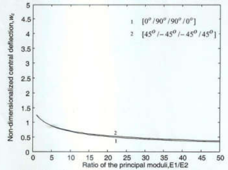
Fig. 4 Effect of material anisotropy on the non-dimensionalized centre deflections of a four layered symmetric cross-ply and angle-ply simply supported laminates (SS5) under uniform lateral load ( \bar{q} = 100.0, h/a = 0.1 ).
