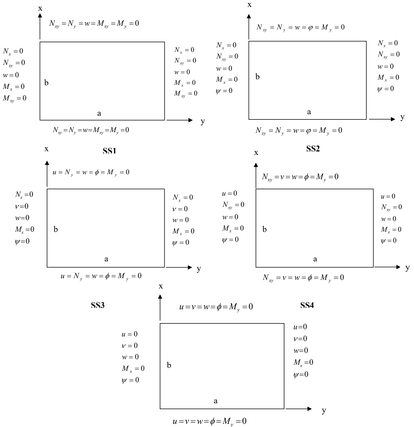
SS5 Fig. (1) Simply supported boundary condition
