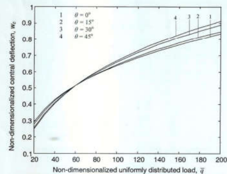
Fig. 6 Variation of central deflection with pressure of simply supported (SS4) antisymmetric square plate of the arrangement [0^\circ/-\theta^\circ/\theta^\circ/-\theta^\circ] with different orientations ( h/a = 0.2 ).
