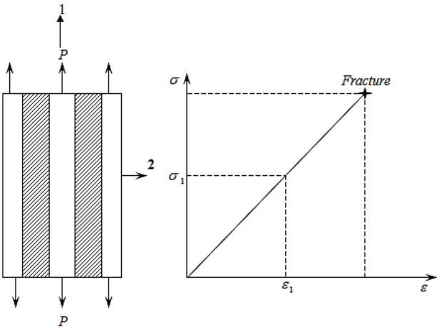
Fig. (1.4) Unidirectional lamina loaded in the fiber-direction
