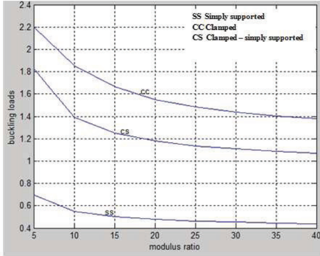
Fig. (5.6) Effect of material anisotropy
