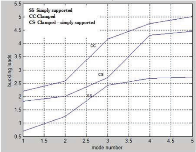
Fig. (5.9) Effect of boundary conditions
