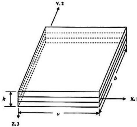
Fig. 3.1 The geometry of a laminated composite plate
