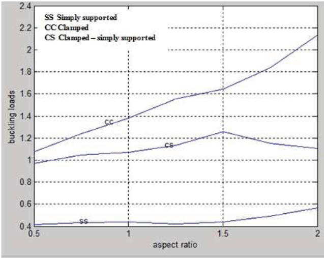
Fig. (5.4) Effect of aspect ratio for different boundary conditions,
