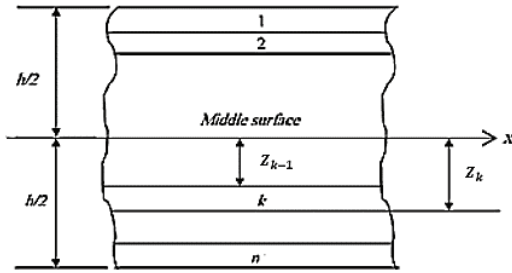
Fig. 3.3 Geometry of an n-layered laminate
