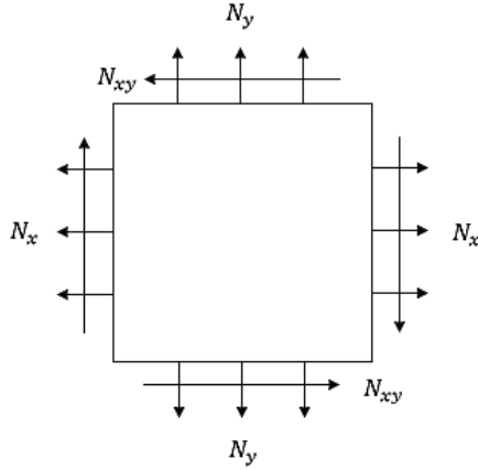
Fig. (3.4) External forces acting on an element
