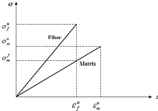
Fig. (1.2) Stress-strain relationships for fiber and matrix
