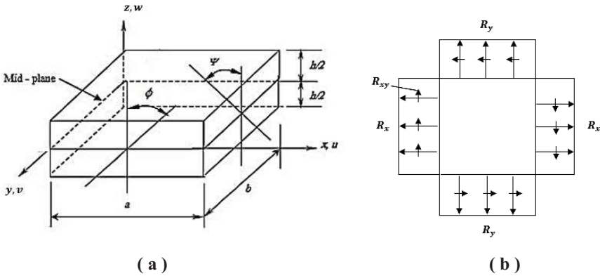
Fig. 3.2 A plate showing dimensions and deformations
