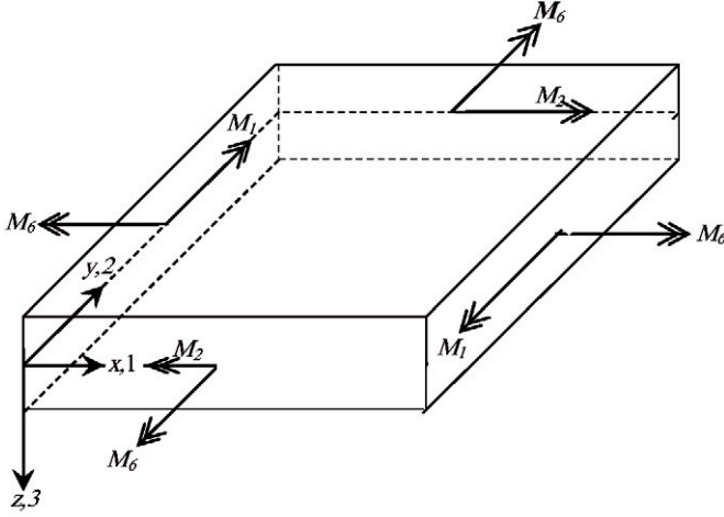
Fig. 2.6 Nomenclature for stress couples
