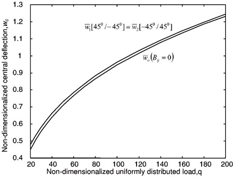
Fig. B.13 Central deflection of a two layer antisymmetric angle-ply simply supported (SS5) rectangular plate under uniform pressure ( b/a = 5.0 , h/a = 0.1 ).
