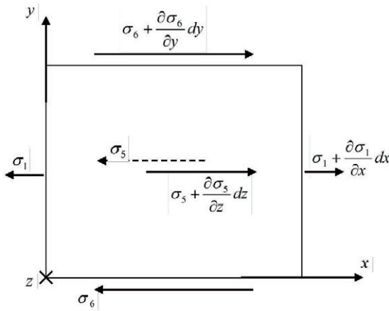
Fig.2.4 Stresses acting in the x -direction.
