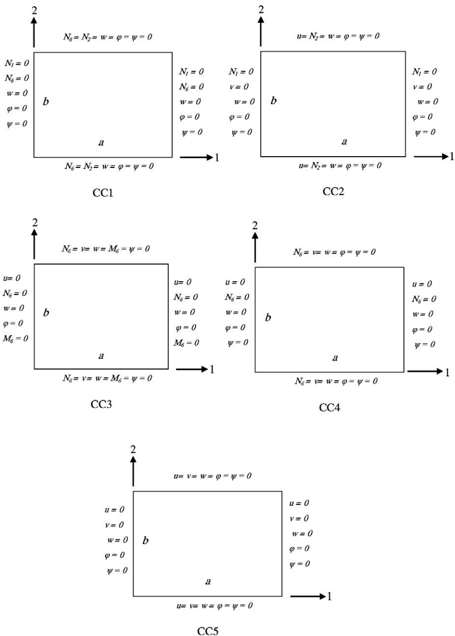
Fig. C.2 Clamped boundary conditions
