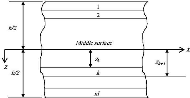
Fig. 2.2 Geometry of an n -Layered laminate
