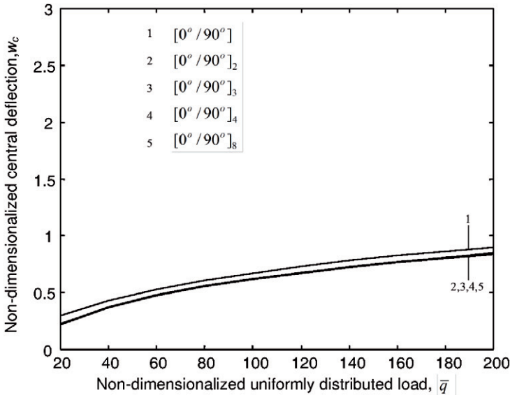
Fig. B.4 Number of layers effect on a simply supported (SS) antisymmetric cross-ply [(0^\circ / 90^\circ)_n] square plate under uniformly distributed loads ( h/a = 0.1 ).
