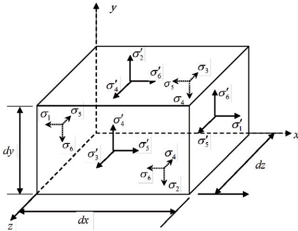
Fig.2.3 Stresses acting on an infinitesimal element
