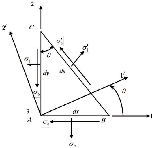
Fig.2.8 Stresses on a triangular element
