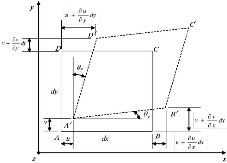
Fig.2.7 Small deformation of an elastic element
