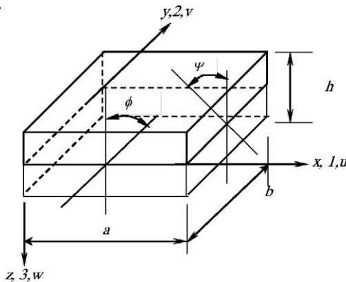
Fig. 2.1 A plate showing dimensions and deformations
