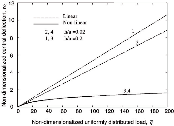
Fig. B.1 Variation of central deflection, \bar{w}_c with load, \bar{q} of thin ( h/a = 0.02 ) and thick ( h/a = 0.2 ) simply supported (SS) square isotropic plate.
