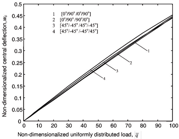
Fig. B.17 Variation of central deflection, \bar{w}_c with pressure, \bar{q} of clamped (CC2) 4-layered anti-symmetric and symmetric cross-ply and angle-ply square laminate ( b/a = 0.1 ).
