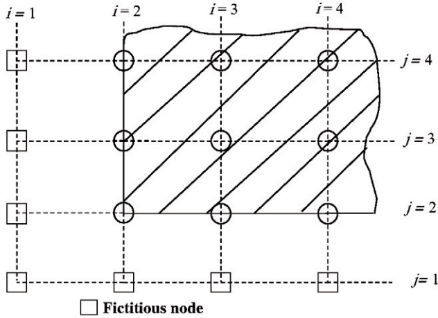
Fig.3.2 Fictitious nodes outside the plate boundaries.
