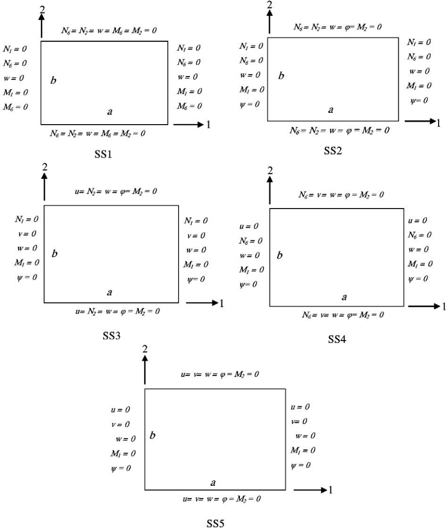
Fig. C.1 Simply supported boundary conditions
