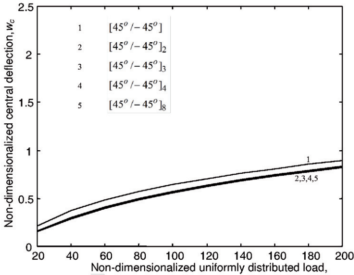
Fig. B.5 Number of layers effect on a simply supported (SSS) antisymmetric angle-ply [(45^\circ / -45^\circ)_n] square plate under uniformly distributed loads ( h/a = 0.1 ).
