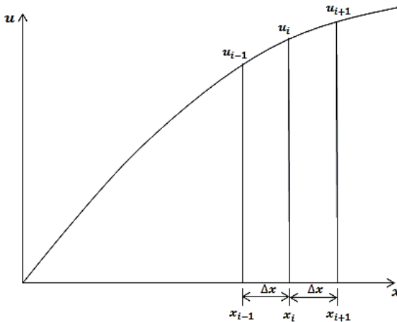
Figure (1.1) Non – uniform or graded mesh
