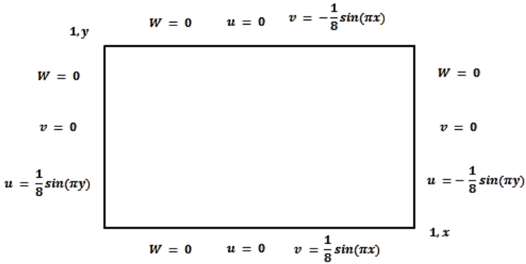
Figure (2.3) Boundary Conditions of Example (2.3)
